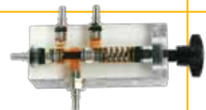
SAI9463 - High - Low pressure circuit
