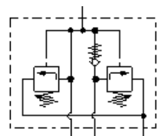
SAI9463 - High - Low pressure circuit
