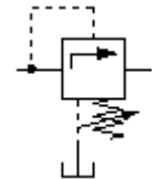
SAI9418 - 3 way pressure relief valve, with damping.
