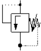
SAI9414 - Pressure relief valve (ball valve), direct control.
