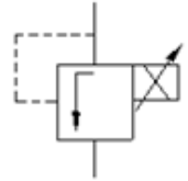
SAI9402 - Proportional pressure relief valve, direct control.
