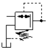
SAI9420 - Pressure reducing valve, 3 way. Direct control.
